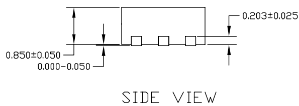
6-Pin 2x2 MLF ® (ML)
